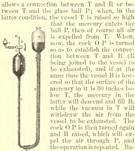
FIG. 5.—Geisler's Mercurial Air Pump.
